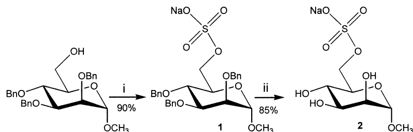
Scheme 1. Reagents and conditions: (i) \text{SO}_3/\text{C}_5\text{H}_5\text{N} , \text{C}_5\text{H}_5\text{N} , 4 h; (ii) \text{H}_2 , \text{Pd}(\text{OH})_2/\text{C} (20%), \text{EtOH}/\text{H}_2\text{O} (1:1), 24 h.
