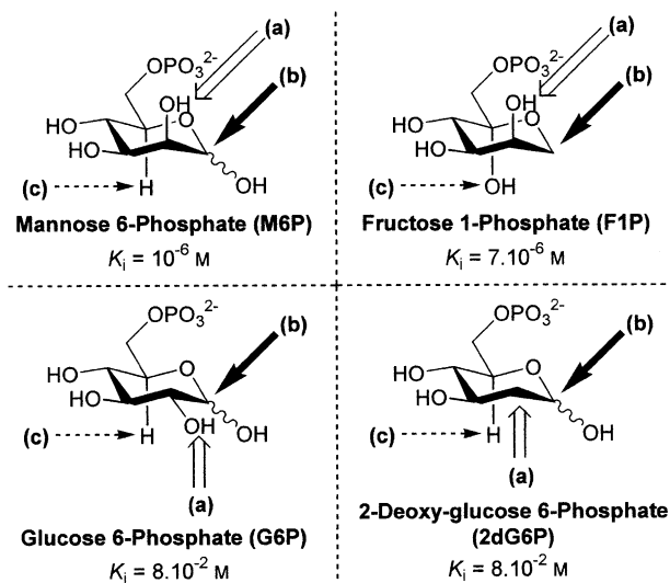
Figure 2. Three main structural requirements for reaching high affinity toward the M6P/IGFIIR. Influence of the substitution at the (a) 2-position, (b) anomeric center and (c) 5-position.
