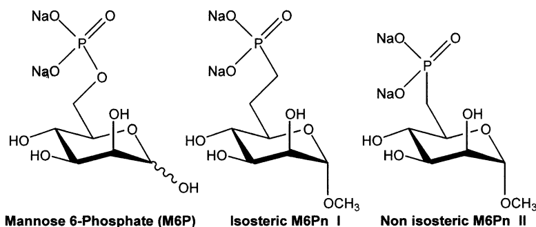
Figure 1. Relation of the distance between the negative charge and the pyranose ring.
