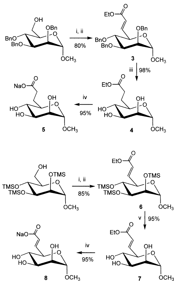
Scheme 2. Reagents and conditions: (i) (\text{COCl})_2 , DMSO, i\text{-Pr}_2\text{NEt} , -60^\circ\text{C} , THF; (ii) (\text{EtO})_2(\text{O})\text{PCH}_2\text{CO}_2\text{Et} , NaH, THF; (iii) \text{H}_2 , \text{Pd}/\text{C} (10%), \text{EtOH}/\text{H}_2\text{O} (1:1), 4 h; (iv) 2 M NaOH, 1 h; (v) HCl (1 M in THF), 5 min.
