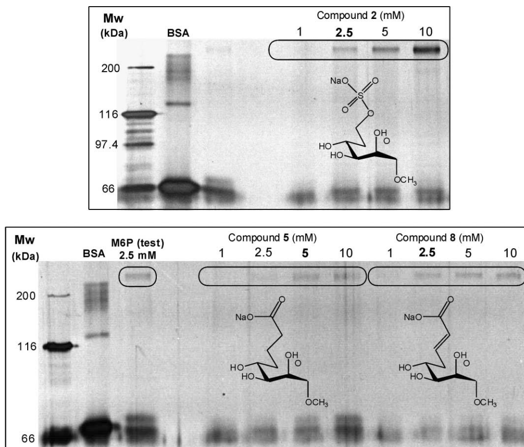
Figure 3. Affinities of M6P analogues toward M6P/IGFIIR. M6P/IGFIIR from calf serum was retained on phosphomannan Sepharose columns and eluted with the indicated concentrations of mannose 6-phosphate (M6P test) and compounds 2 , 5 and 8 . The eluted protein was analyzed in a 10% SDS polyacrylamide gel followed by silver-staining. Mw, molecular weight markers; boxes indicate the eluted M6P/IGFIIR.
